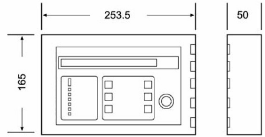
ZXr-A and ZXr-P Dimensions
